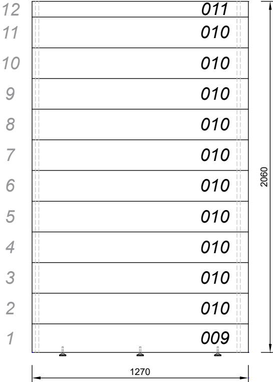
WALL A (LEFT) VIEW FROM THE OUTSIDE
