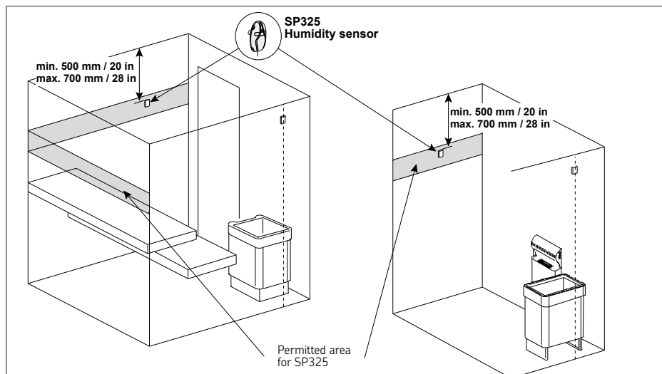
Fig. 8: Installation bench sensor
