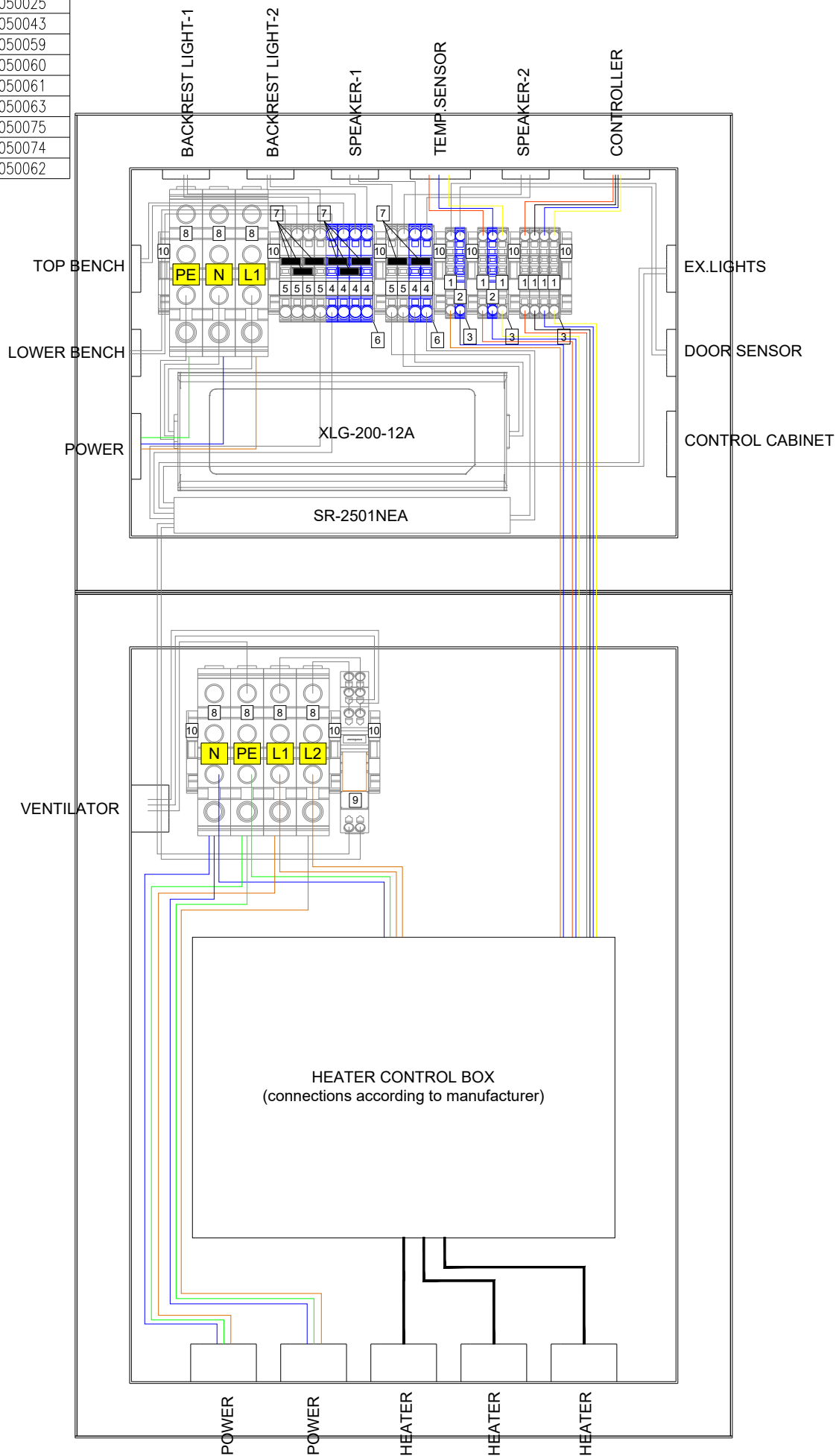
Figure 2. SAUNALIFE G7 CONNECTIONS AFTER SAUNA INSTALLATION
