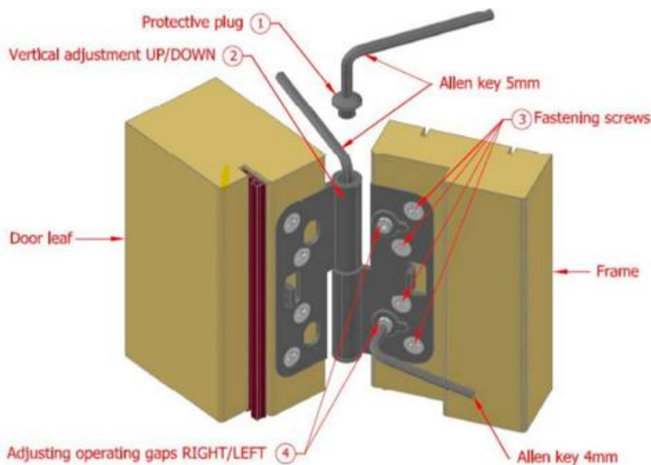
Figure 3. Adjusting the hinges
