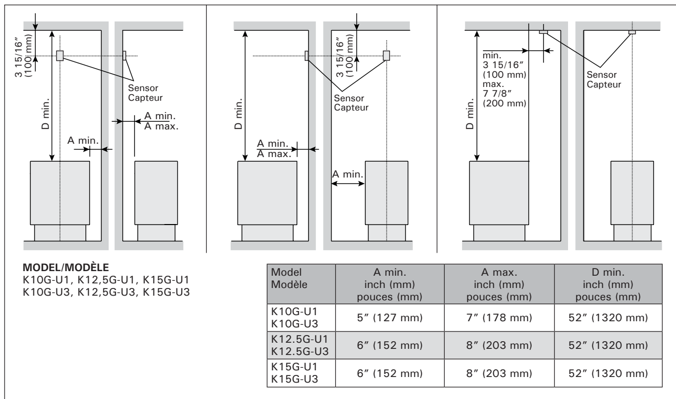
Figure 8. The place of the temperature sensor of the control unit in connection with floor-mounted heaters
