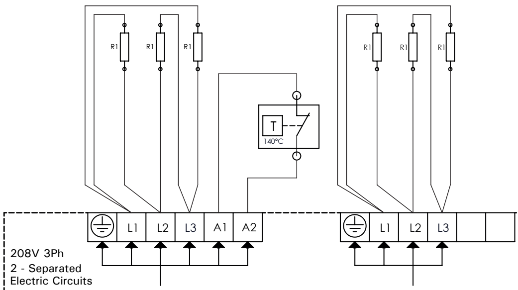
Figure 6. Electrical connections of heater
