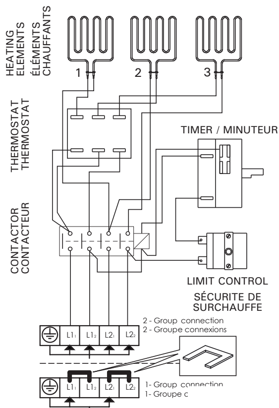
Figure 5. Electrical connections of the heater
