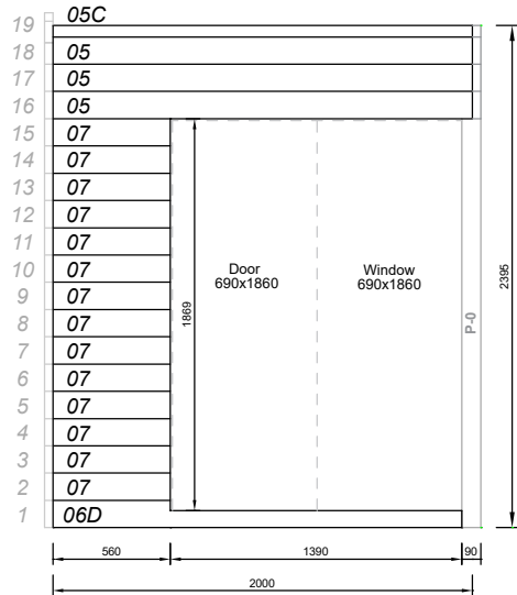
Wall 2 (front) View from the outside
