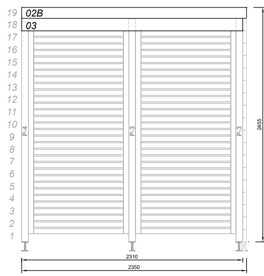
Wall C (right) View from the outside
