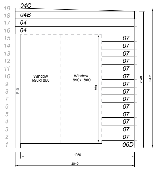
Wall B (right) View from the outside
