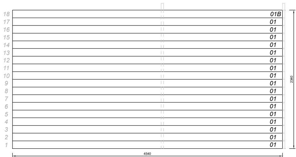
Wall B (right) View from the outside
