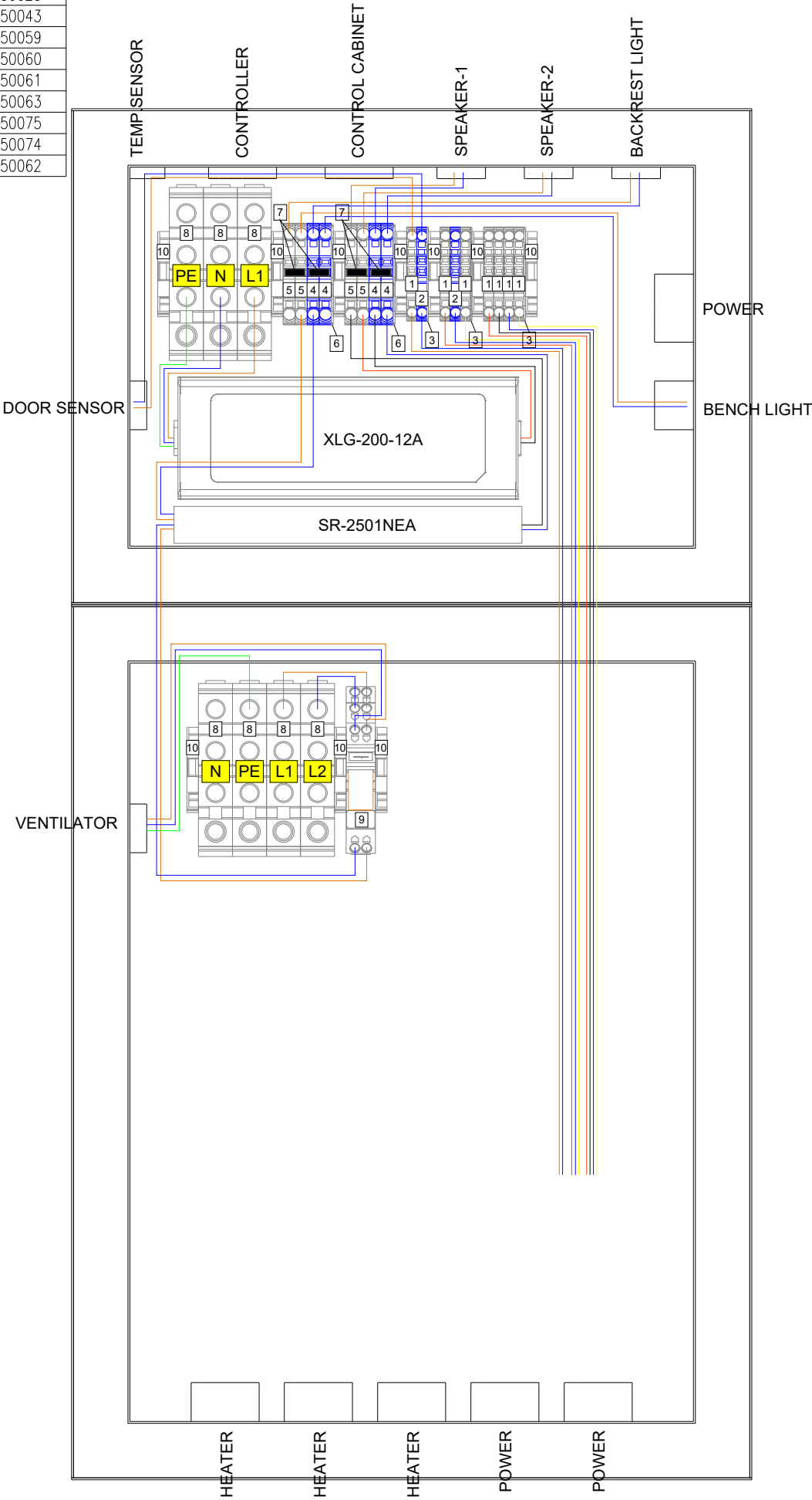
Figure 1. SAUNALIFE G6 CONNECTIONS DONE IN FACTORY
