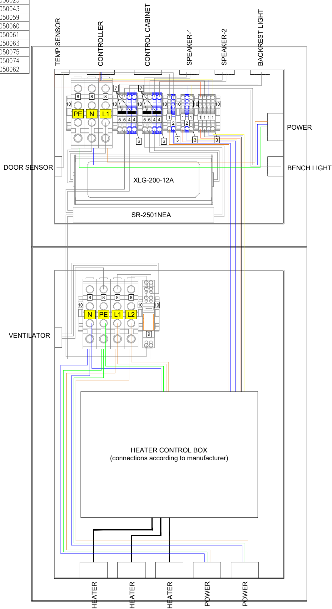
Figure 2. SAUNALIFE G6 CONNECTIONS AFTER SAUNA INSTALLATION
