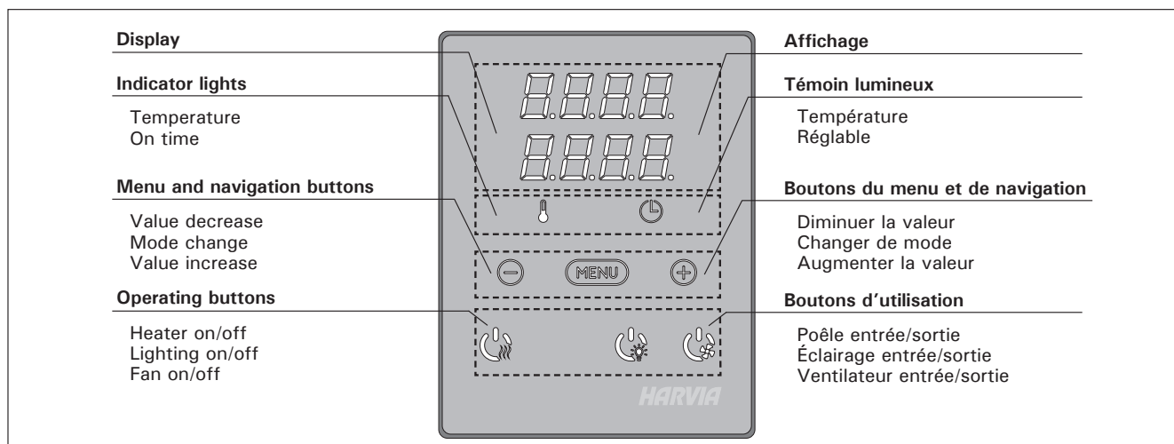
Figure 2. Control panel
